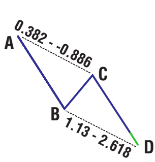
Bullish AB=CD
